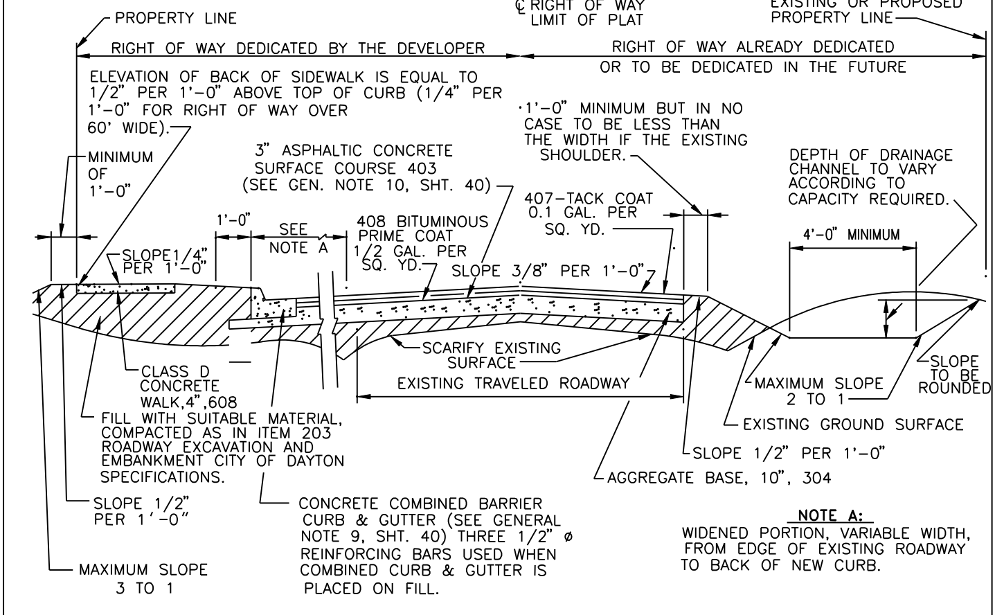
TYPICAL SECTION FOR HALF STREET DEDICATIONS OF STREET CONSTRUCTED ON FILL NO SCALE
