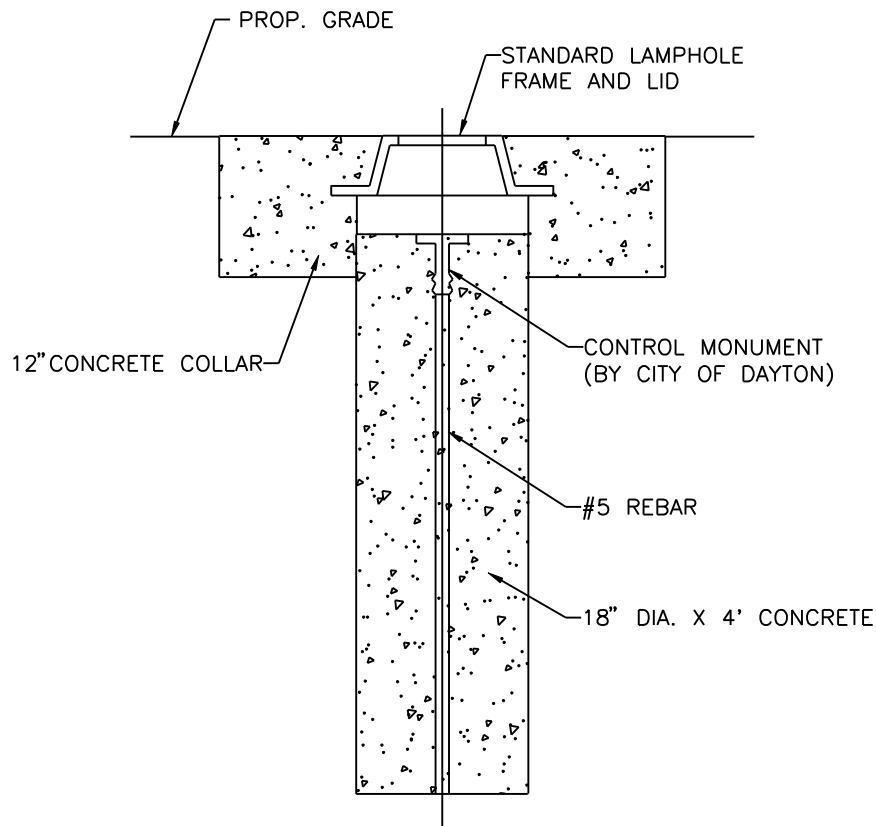
CENTERLINE CONTROL MONUMENT NO SCALE
