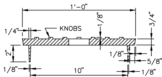
SECTION C-C
