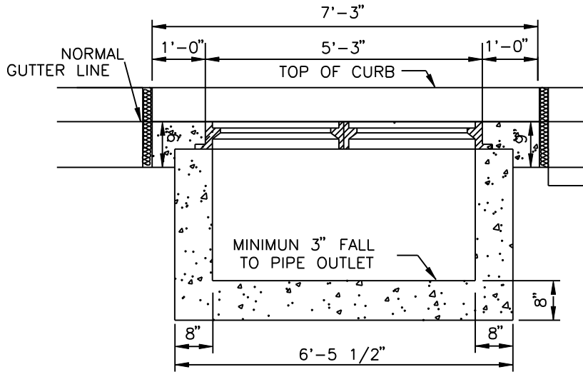
SECTION J-J
