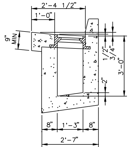
SECTION H-H
