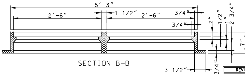
FRAME FOR TYPE C CATCH BASIN
