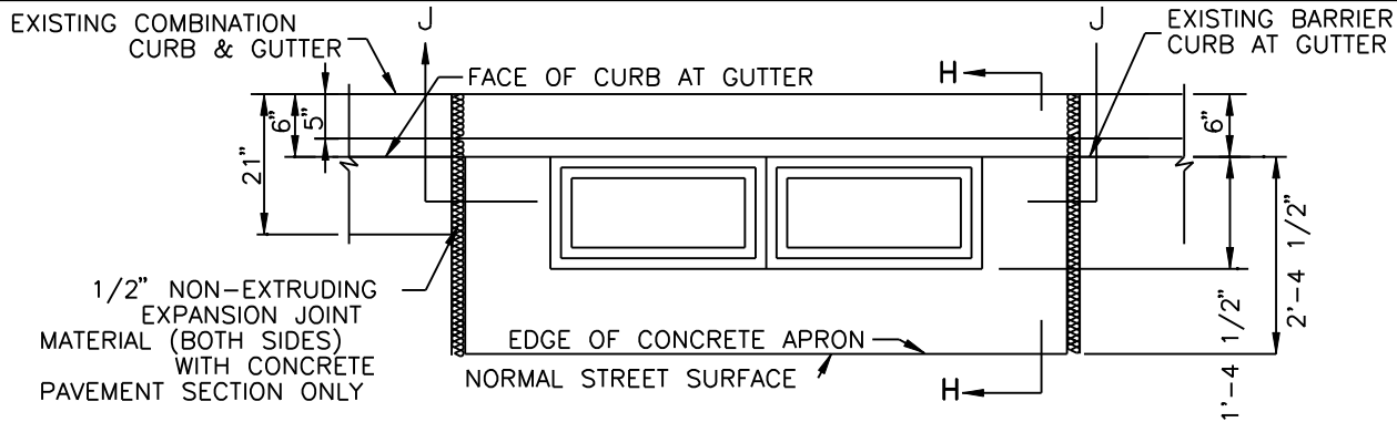
PLAN (WITH GRATING REMOVED)
