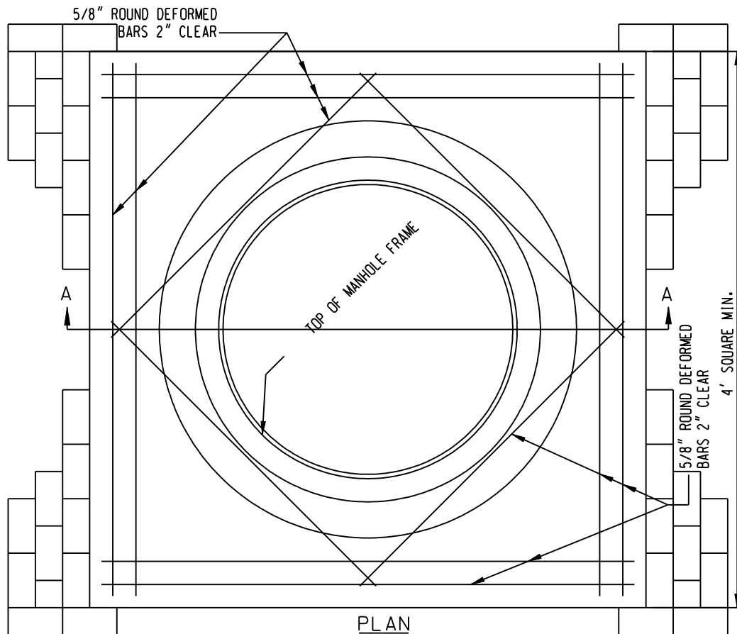
TYPICAL CONSTRUCTION AROUND MANHOLE FOR PAVEMENT USING PAVERS
