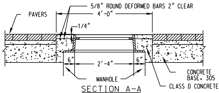
TYPICAL CONSTRUCTION AROUND MANHOLE FOR PAVEMENT USING PAVERS
