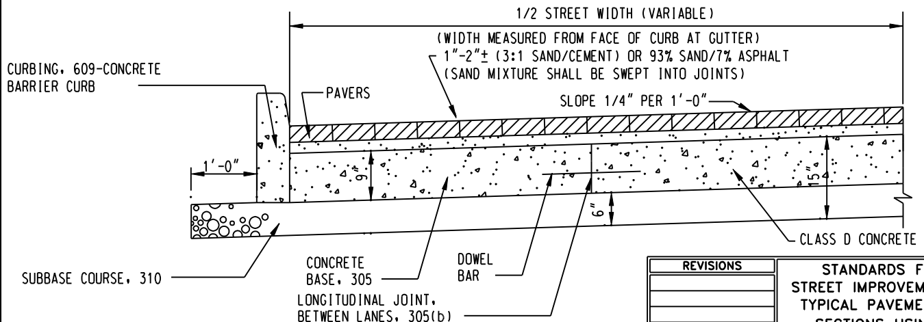
TYPICAL HALF SECTION FOR STREET PAVEMENT USING PAVERS
